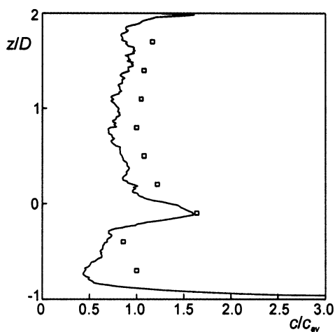
Figure 12. Phase-averaged particle concentration in the plane midway between two baffles as a function of the vertical position in the tank at 2\eta/T = 0.7 for case No. 2B (drawn line), and for experiments reported by Micheletti et al. (2003) with glass beads in the size range 0.3–0.425 mm (symbols).
