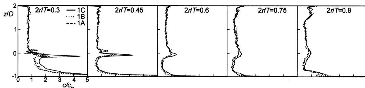
Figure 5. Phase-averaged particle number concentration in the plane midway between two baffles as a function of the vertical position in the tank at five different radial positions.
